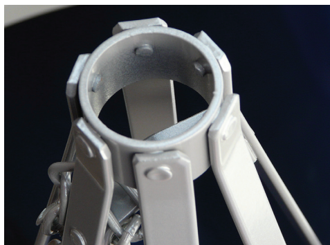
Collar with riveted end fixing.
