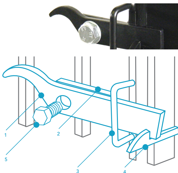
Code MCGR122 Double Gate Catch £0.90 ex VAT £1.08 inc VAT
